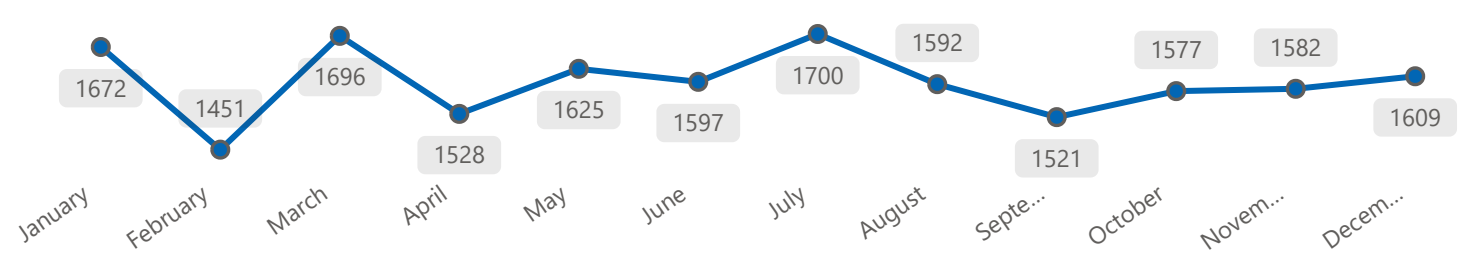
Total_Quantity by Month
